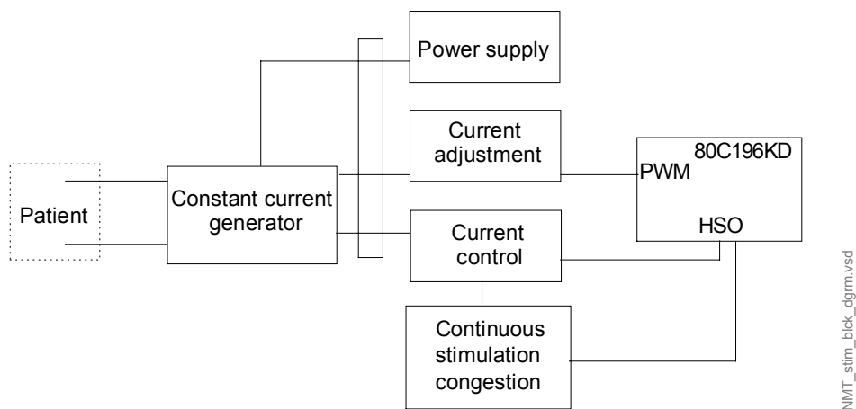
Figure 4 Stimulator block diagram
