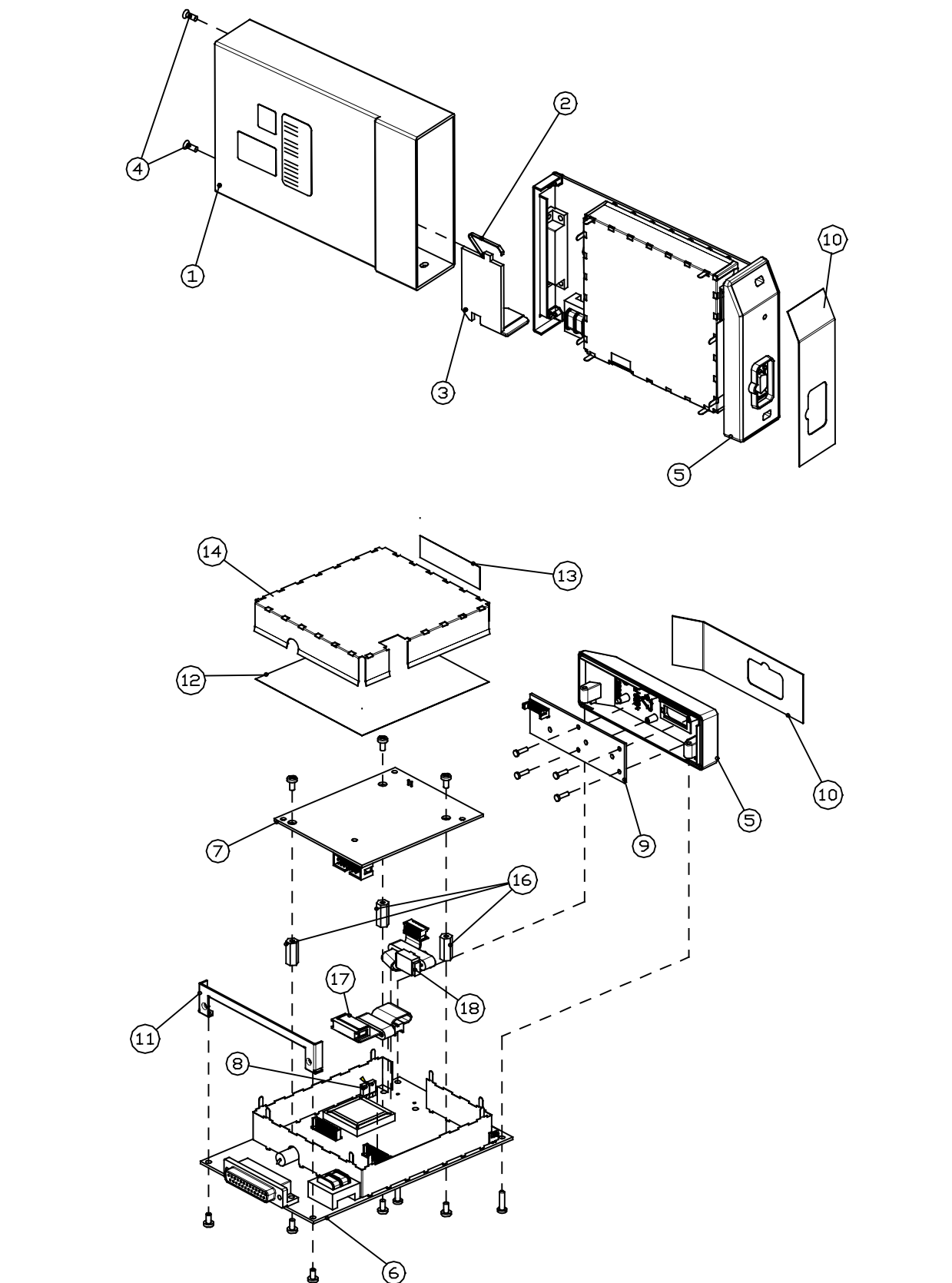
Figure 7 Exploded view of M-NSAT Rev. 04
