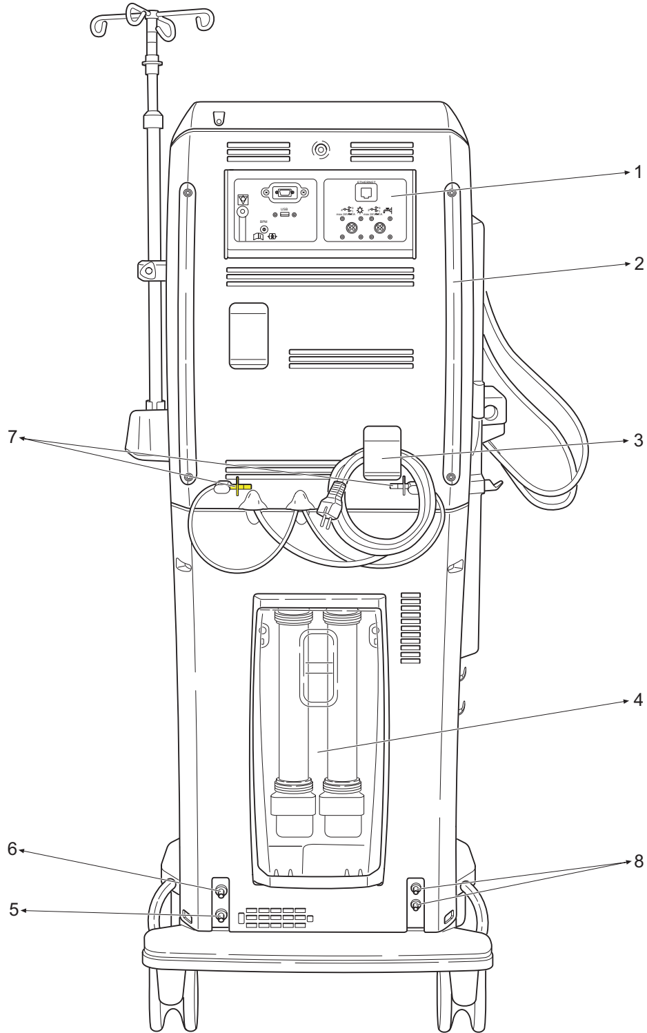
Figure 1-5. Rear Panel
