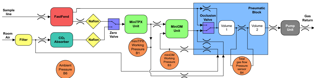
Figure 9 Gas tubing layout
