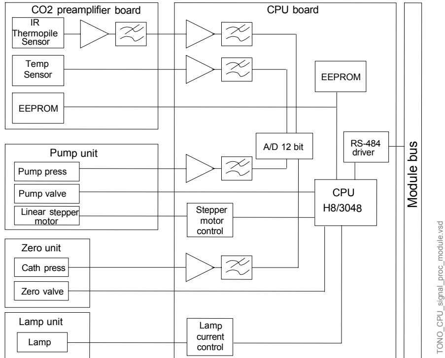
Figure 6 Signal processing of the module
