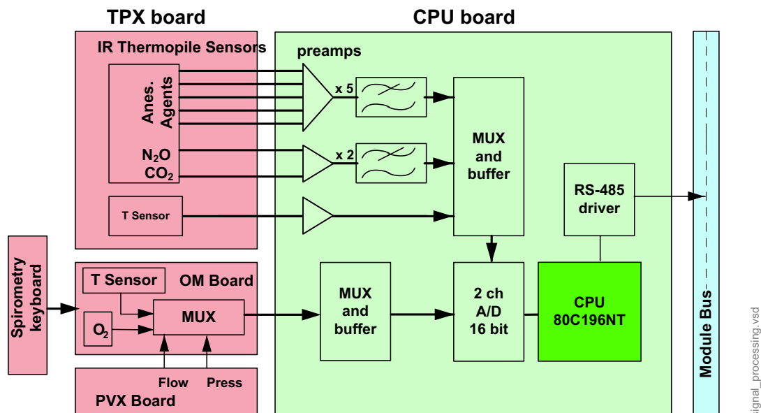
Figure 12 Signal processing
