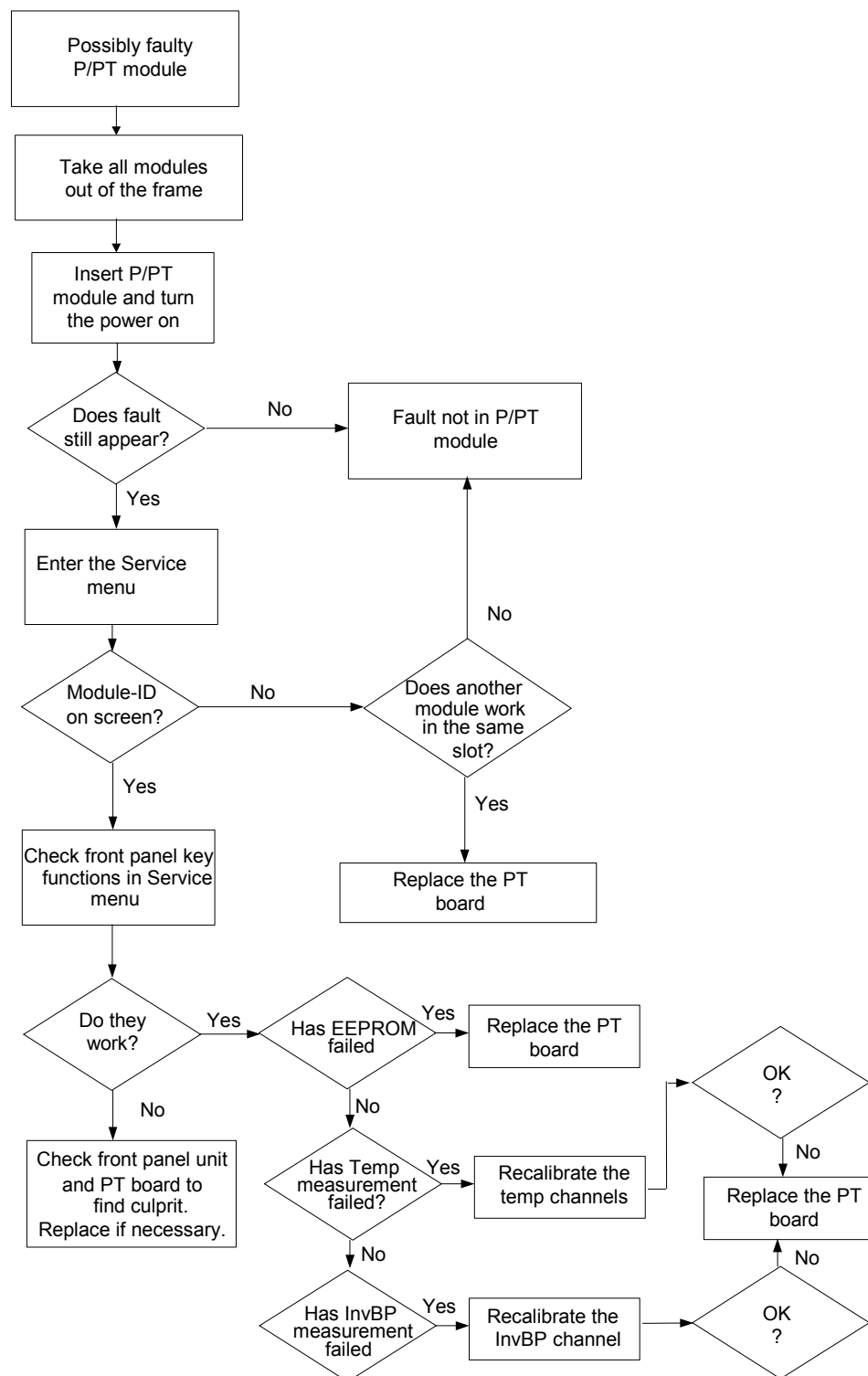
Figure 8 Troubleshooting flowchart
