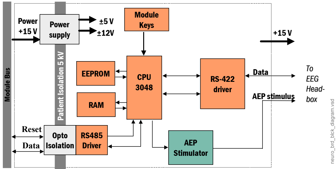
Figure 4 Neuro board block diagram
