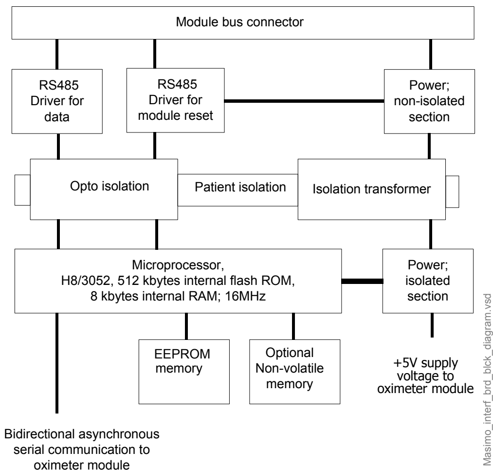
Figure 2 E-MASIMO Interface board block diagram
