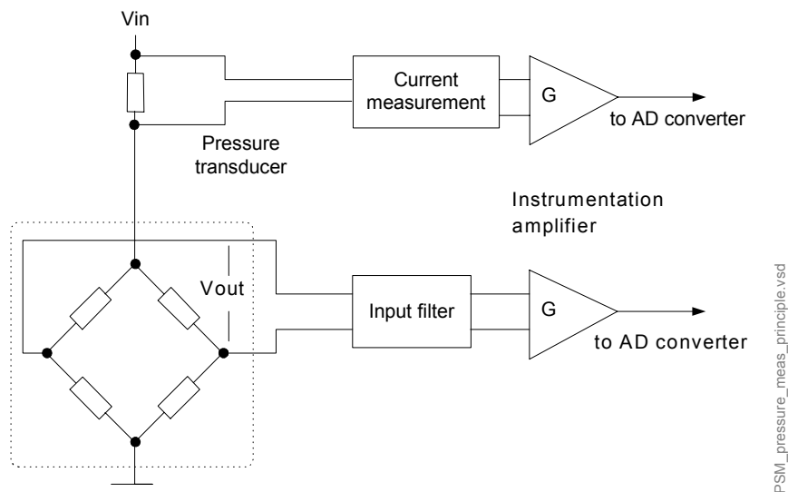
Figure 4 Pressure measurement principle
