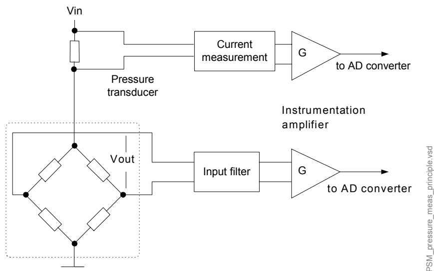
Figure 6 Pressure measurement principle
