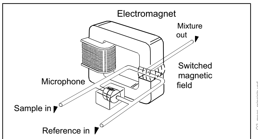
Figure 4 \text{O}_2 measurement principle
