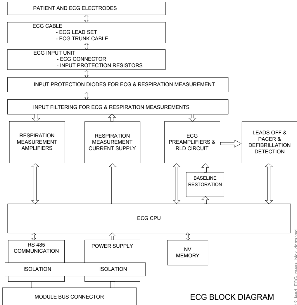
Figure 7 12-lead ECG measurement block diagram
