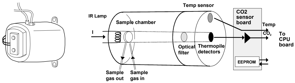
Figure 5 CO 2 sensor
