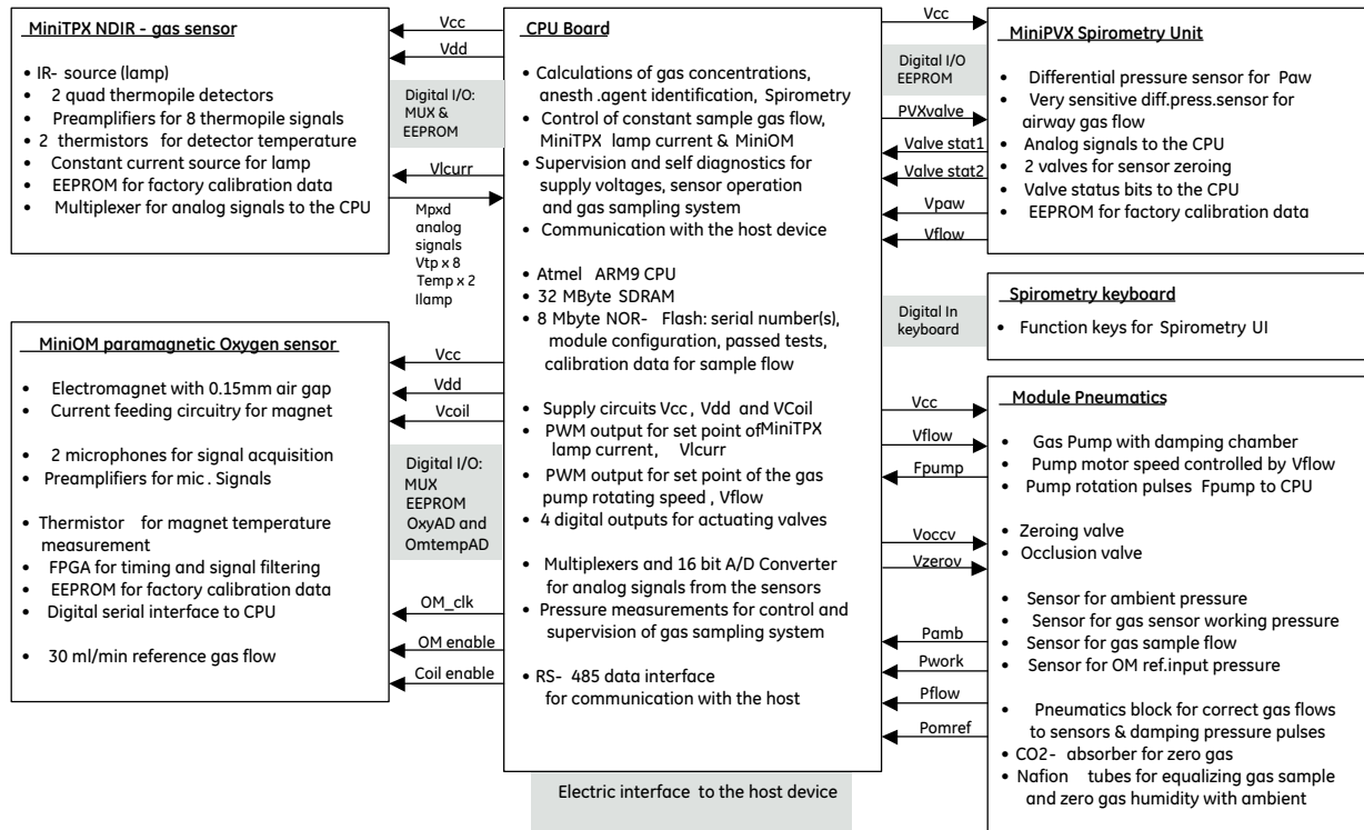
Figure 14 Block diagram
