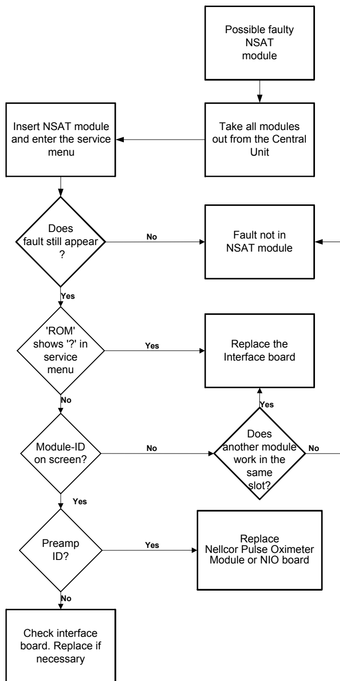
Figure 5 Module troubleshooting flowchart
