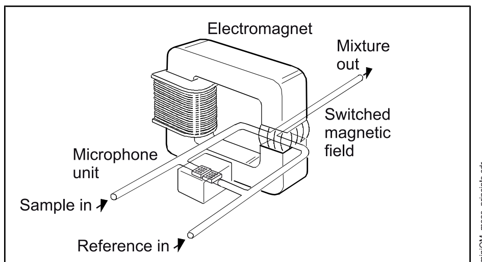
Figure 5 O 2 measurement principle
