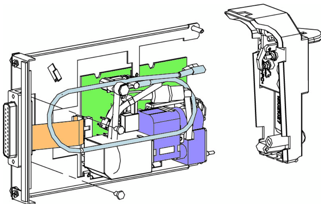
Figure 5 Uncovered E-miniC module
