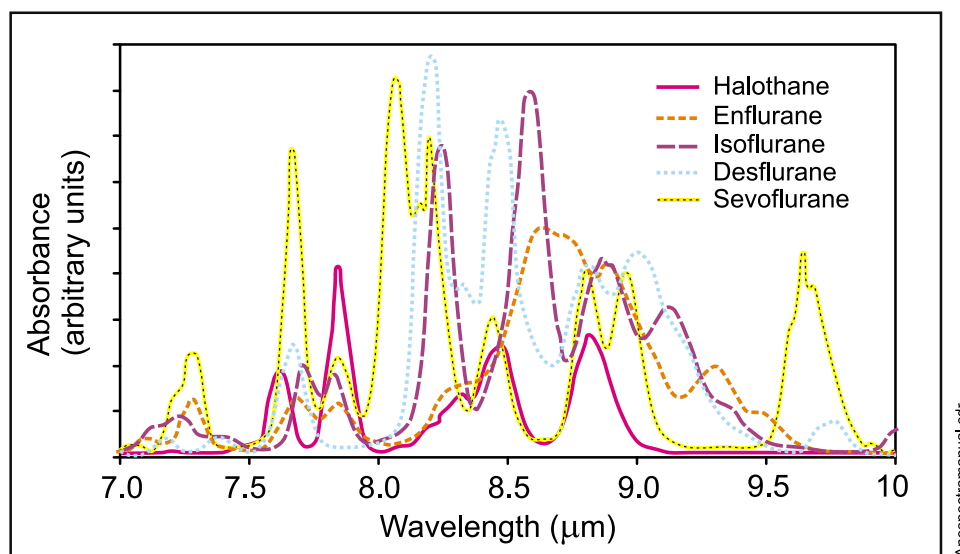
Figure 4 Infrared absorbance of AAs
