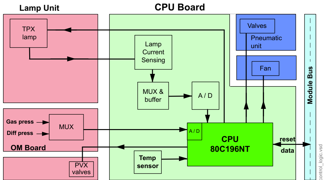
Figure 13 Control logic
