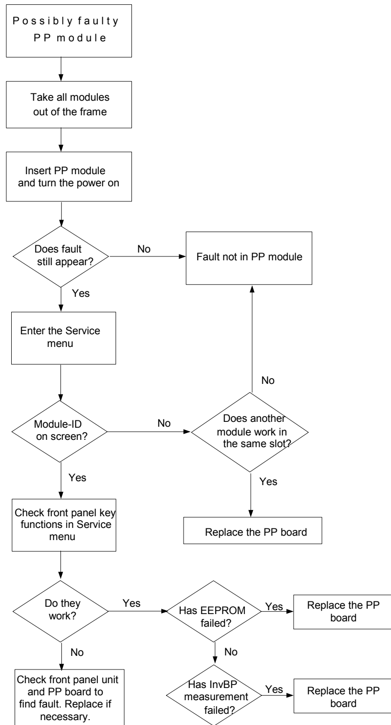
Figure 6 E-PP troubleshooting flowchart
