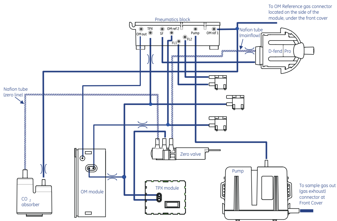
Figure 7 Gas sampling system
