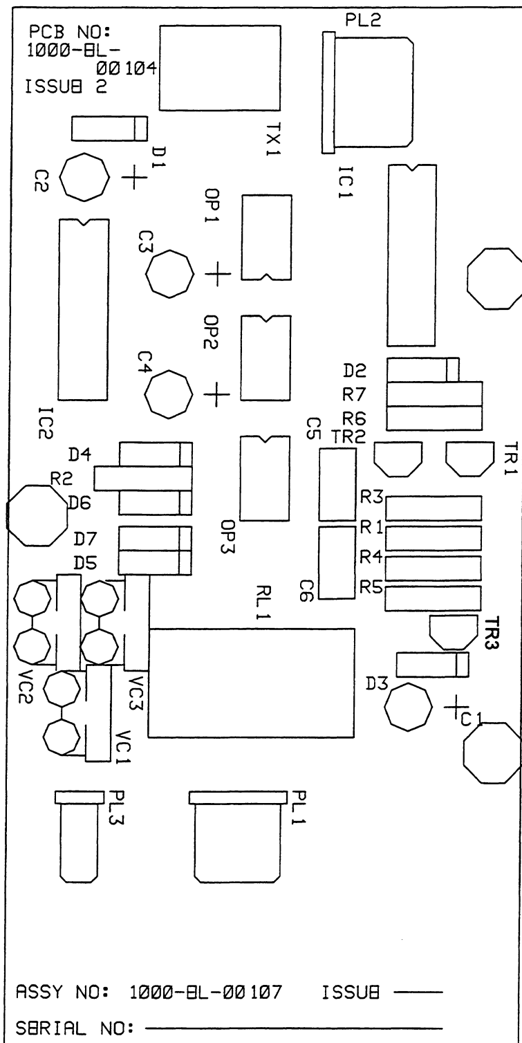
RS232/Nursecall Component Location 1000EL00102 (not issue controlled)
