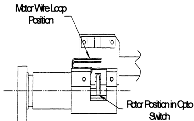
Figure 2. Routing of motor wires between opto mount and flexible circuit.
