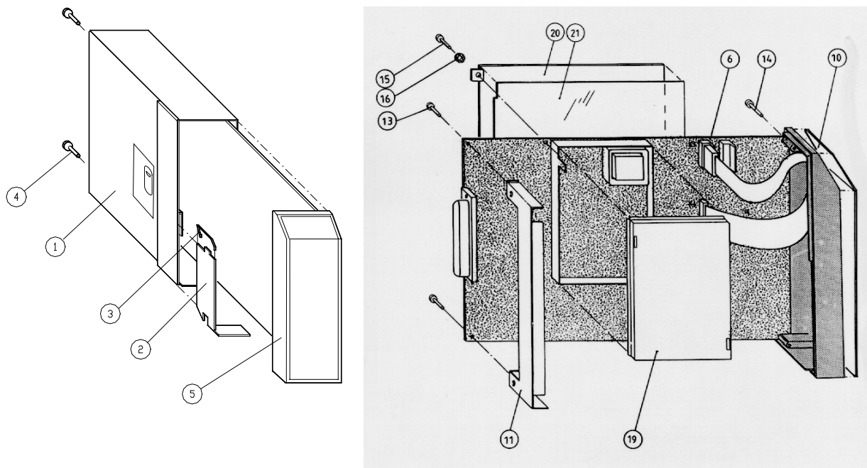
Figure 9 Exploded view of the M-P module
