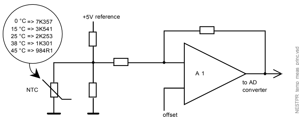
Figure 5 Temperature measurement principle
