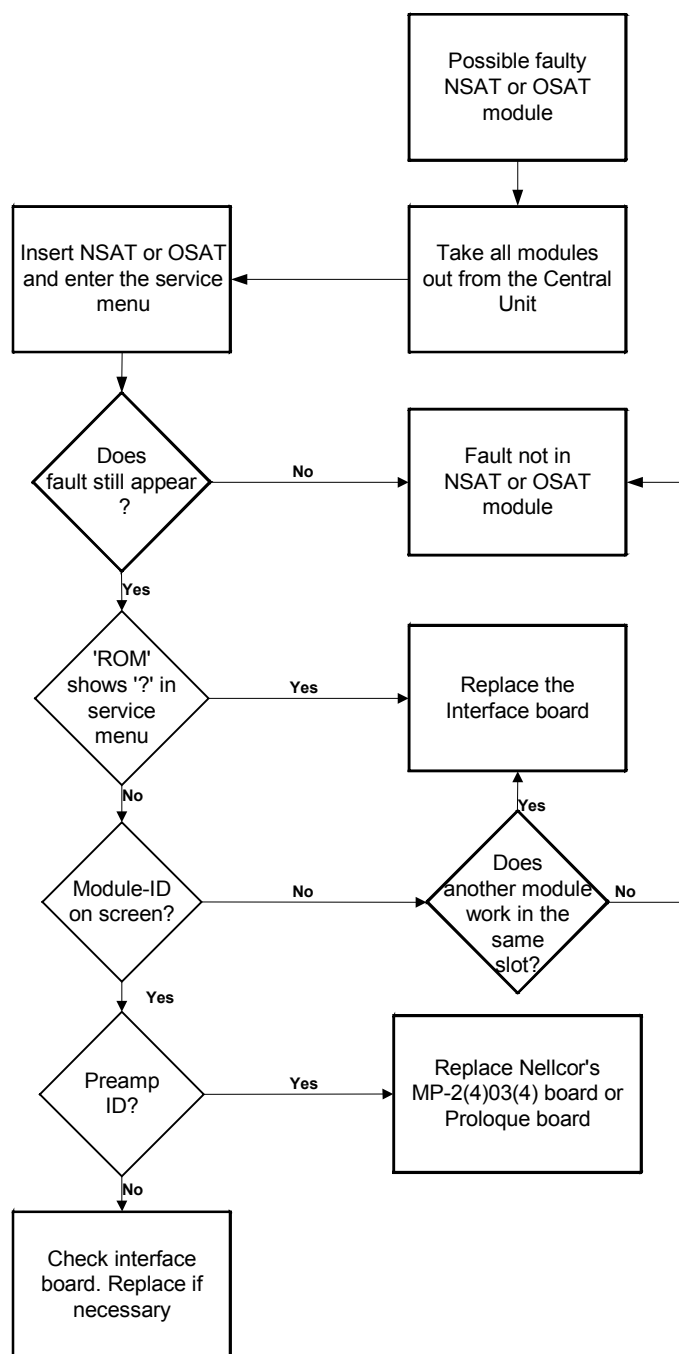
Figure 4 Module troubleshooting flowchart
