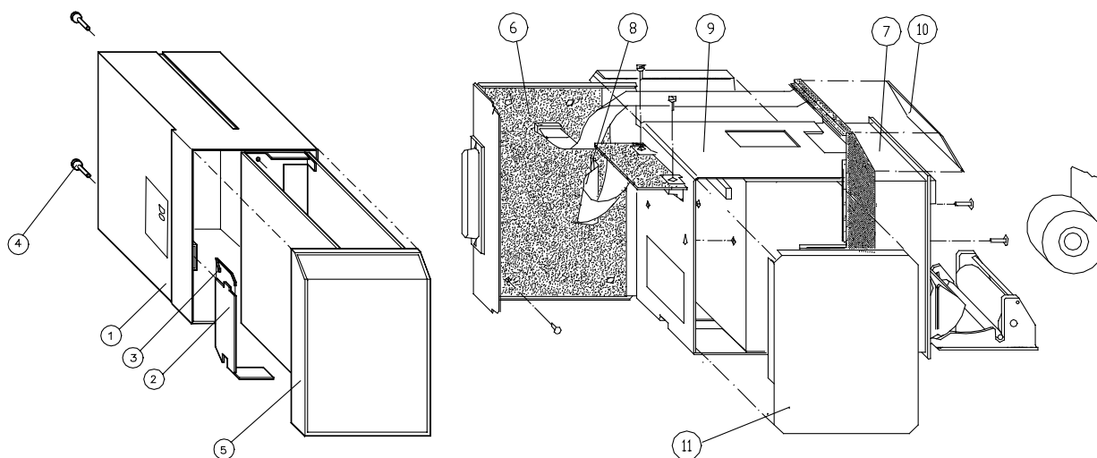
Figure 4 Exploded view of Recorder Module box and Recorder Module
