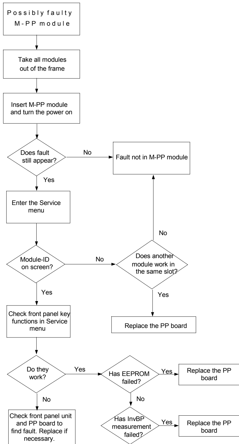
Figure 7 M-PP troubleshooting flowchart
