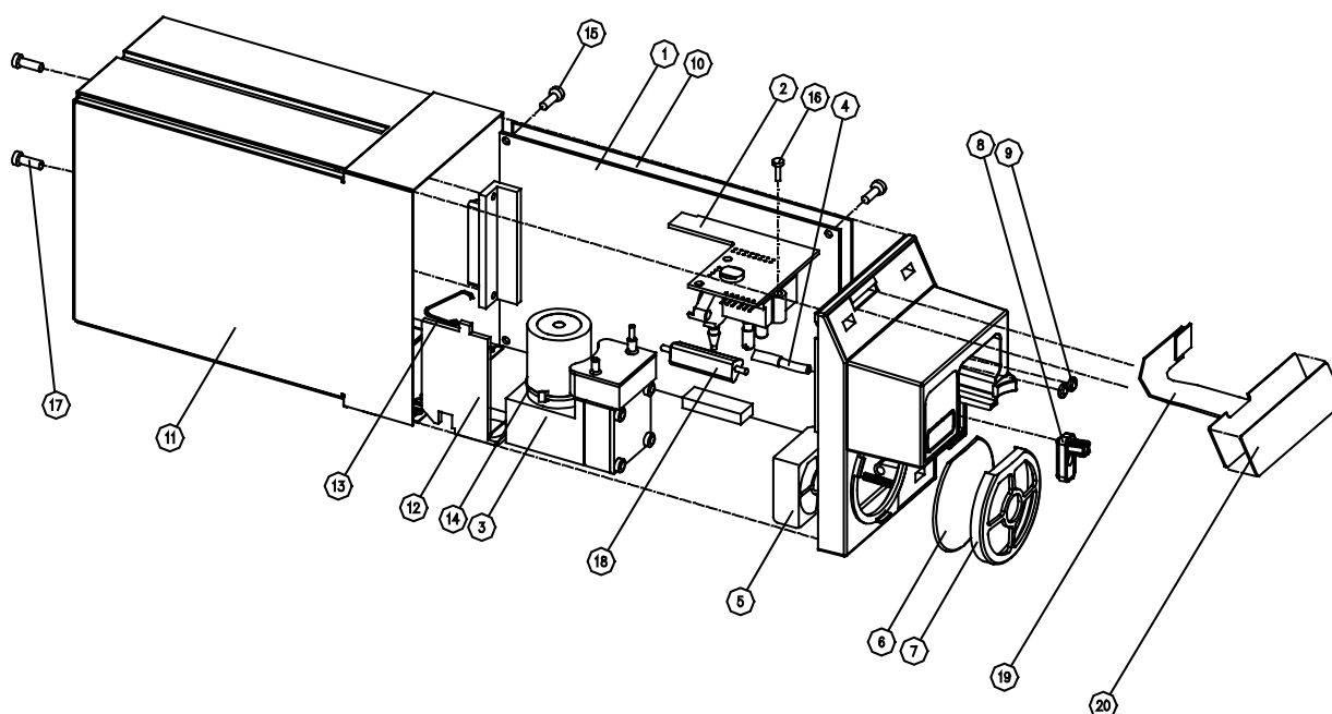
Figure 21 Exploded view M-C rev. 01-02, M-CO rev. 01-03, M-COV rev.03, M-COVX rev.02, M-CAiO rev.02, M-CAiOV rev. 03, M-CAiOVX rev.01
