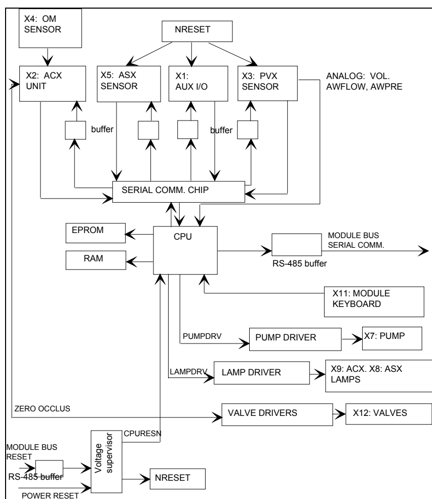
Figure 15 Gas mother board block diagram
