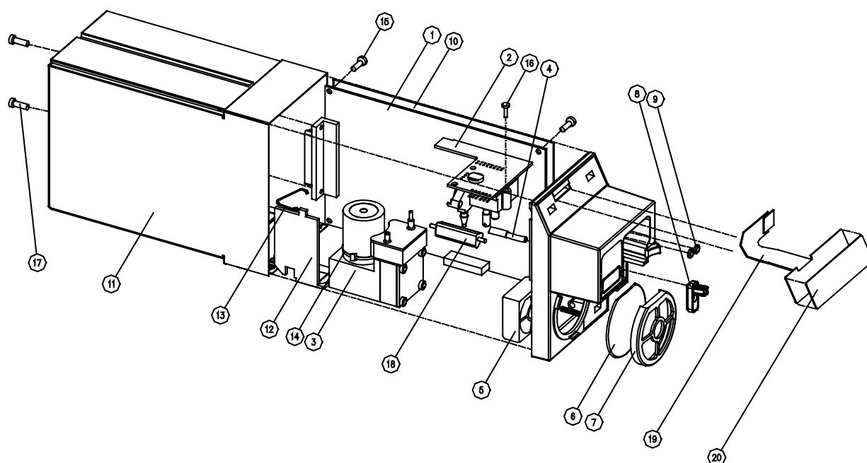
Figure 23 Exploded view M-C rev. 01-02, M-C0 rev. 01-03, M-COV rev.04, M-COVX rev.03, M-CAi0 rev.03, M-CAi0V rev. 04, M-CAi0VX rev.02
