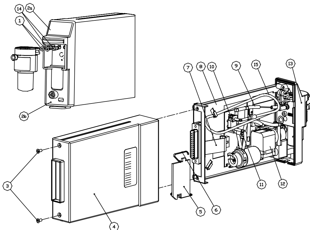
Figure 8 Exploded view of M-miniC
