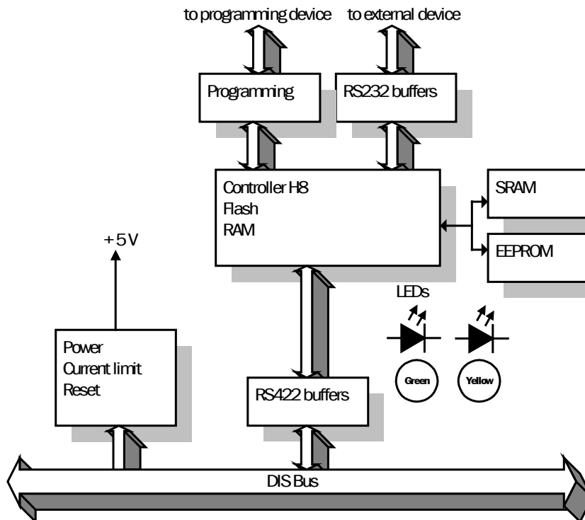
Figure 3 DIS module
