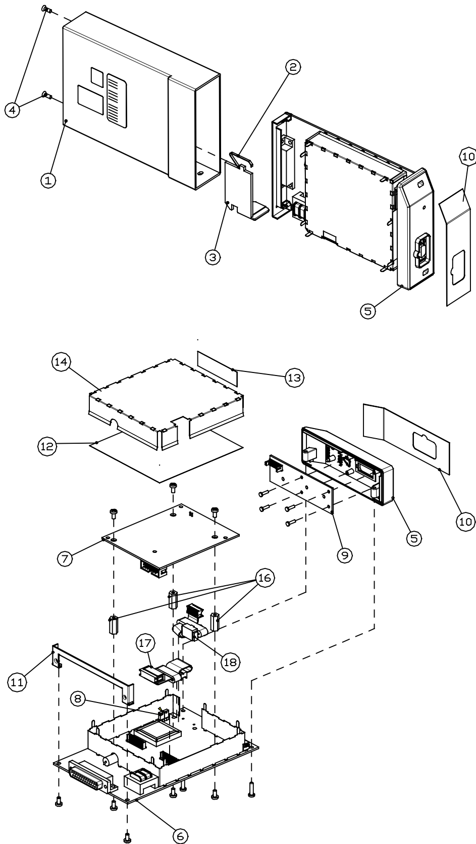
Figure 7 Exploded view of M-NSAT Rev. 04
