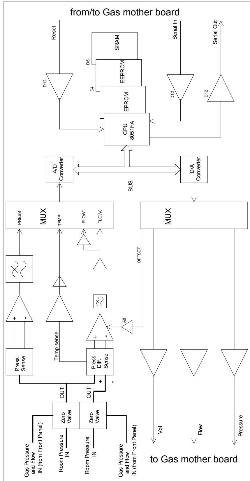
Figure 14 PVX board block diagram
