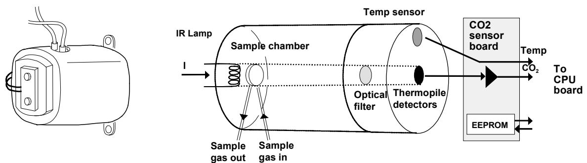
Figure 4 CO 2 sensor
