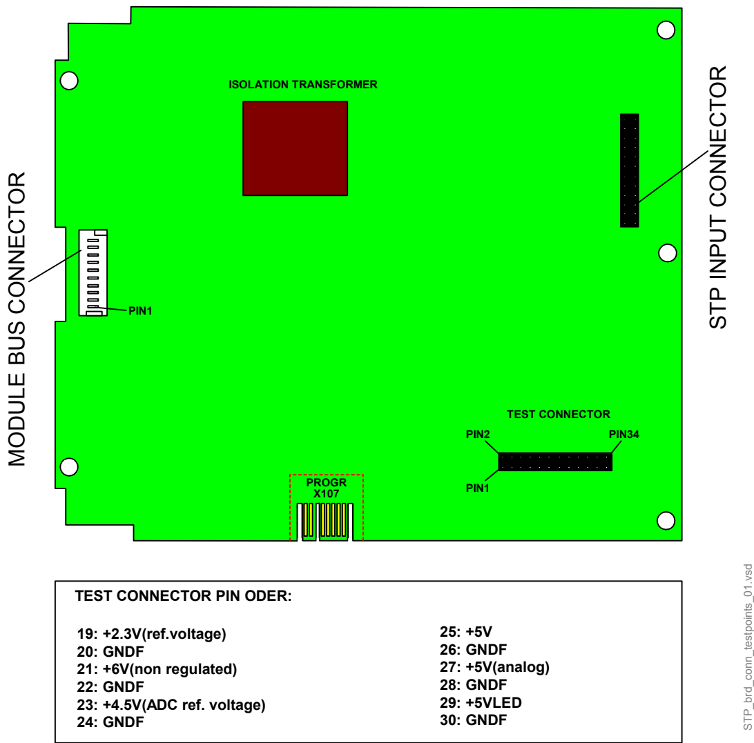
Figure 17 STP board connectors and test points
