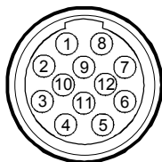
12-lead ECG connector
