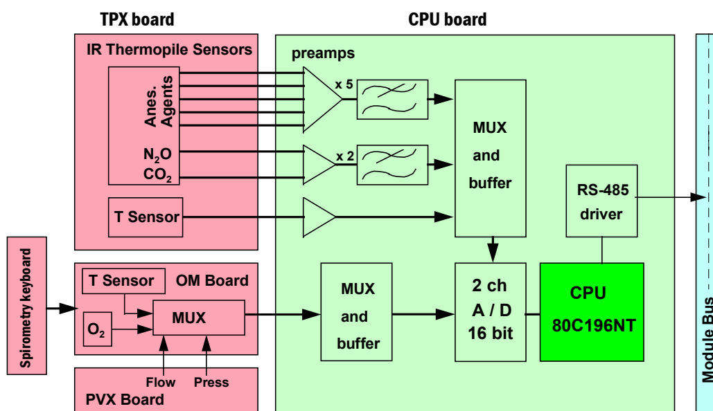
Figure 12 Signal processing
