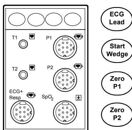
Figure 3 Front panel of M-ESTPR
