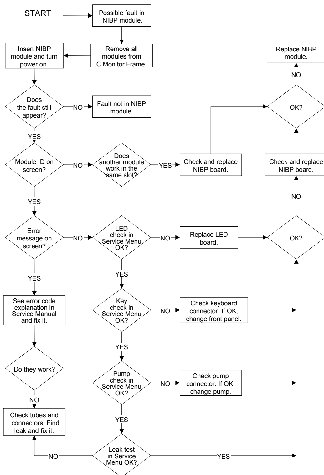
Figure 4 NIBP Module troubleshooting flowchart
