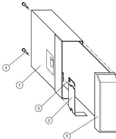
Figure 5 Exploded view of M-NSAT single module
