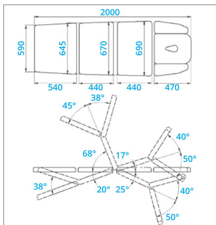
NSR 4 E - electric height adjustment
