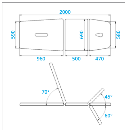
KSR F - manual height adjustment
