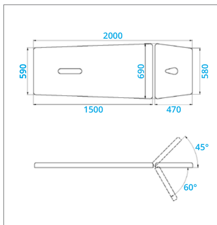
NSR 2 - manual height adjustment
