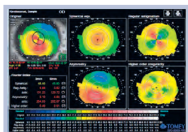
Fourier analysis
