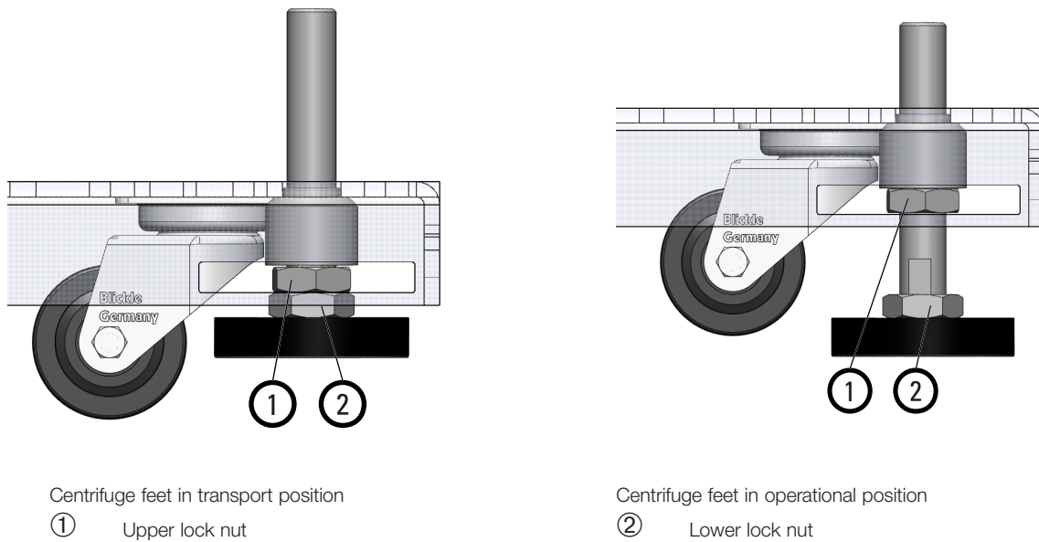
Figure 7: Securing the centrifuge feet
