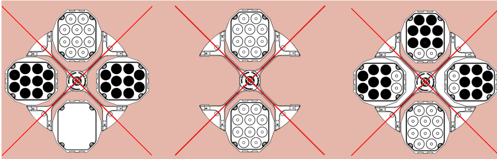
Figure 19: Incorrect loading examples for swinging bucket rotors (simplified top view)
