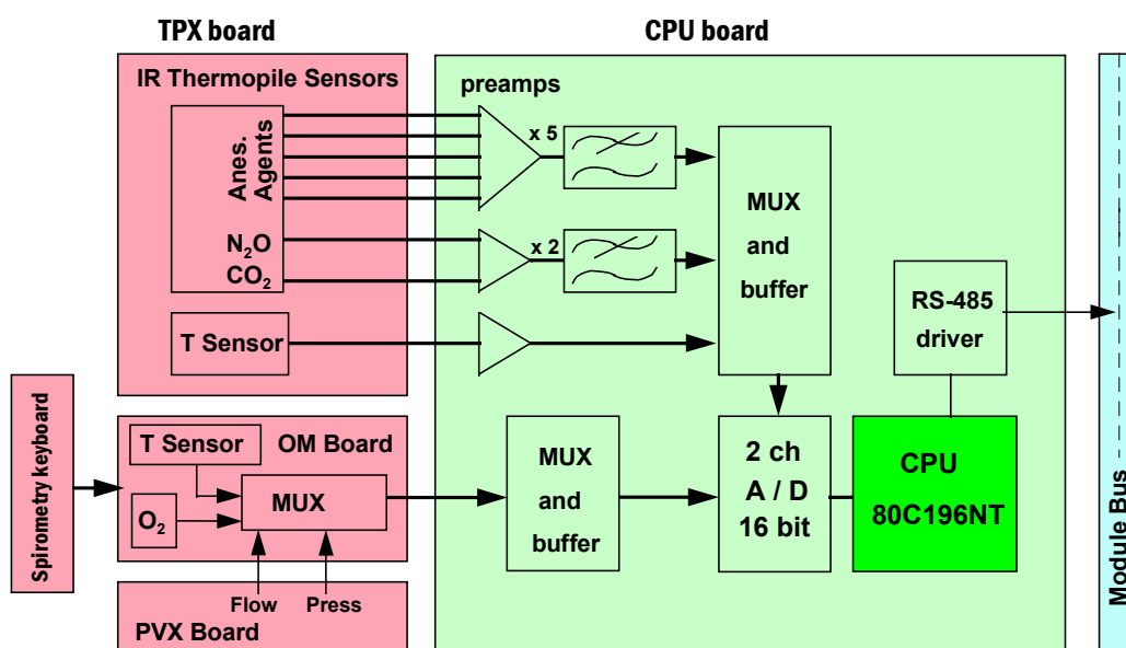
Figure 12 Signal processing
