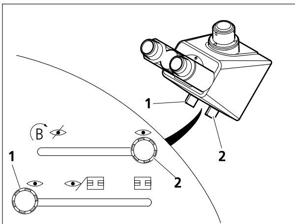
Fig. 3-4 Binocular phototube 45°/23
