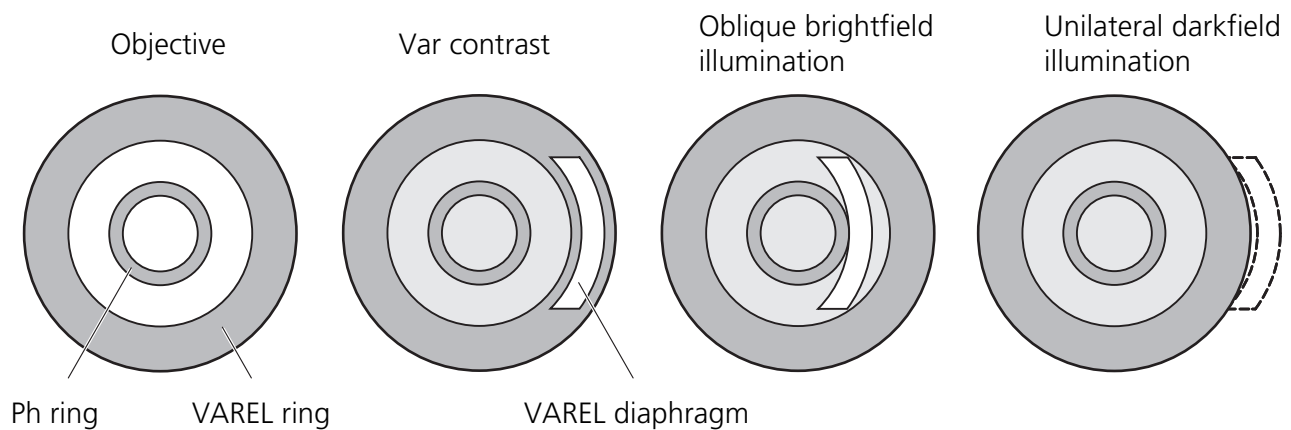
Fig. 3-23 Pupil images in VAREL contrast
