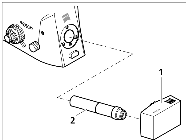
Fig. 3-26 Video attachment
