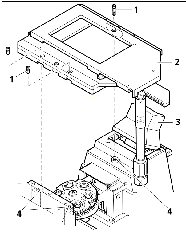
Fig. 2-8 Attachment of mechanical stage 130x85
