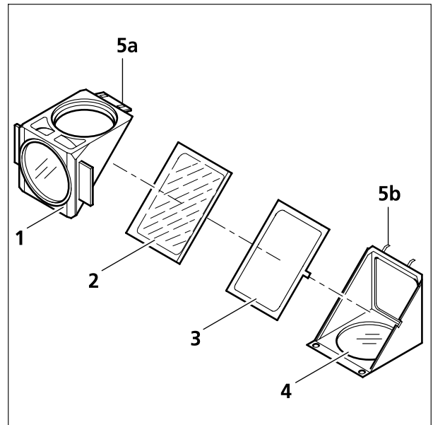
Fig. 2-20 Changing the beam splitter
