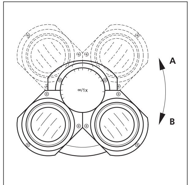
Fig. 3-5 Setting of eyepiece distance on the binocular tube
