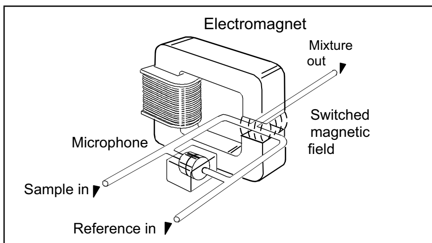
Figure 4 O 2 measurement principle
