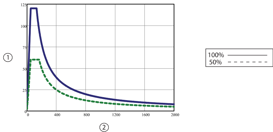
Output power versus impedance for SOFT COAG power
