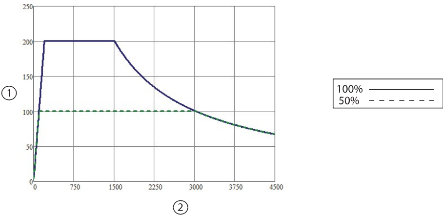
Output power versus impedance for VALLEYLAB power
