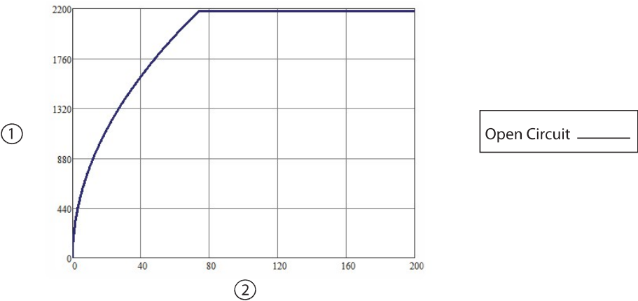
Peak voltage versus power setting for BLEND power
